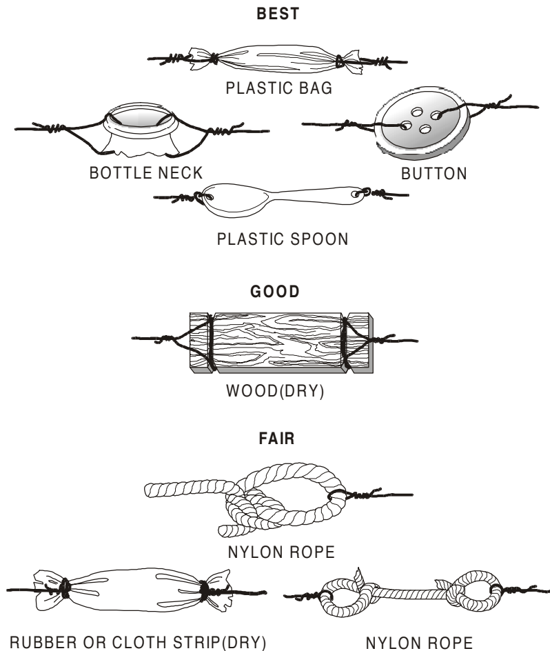
Figure O-2. Improvised Insulators.
