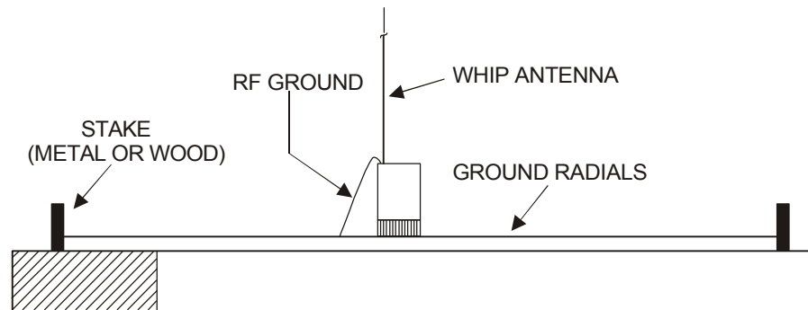
Figure 3-17. Equipment Configuration.
