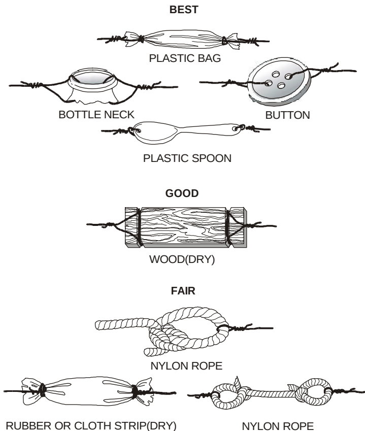
Figure 6-2. Improvised Insulators.
