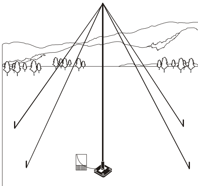
Figure 4-4. AS-2259/GR.
