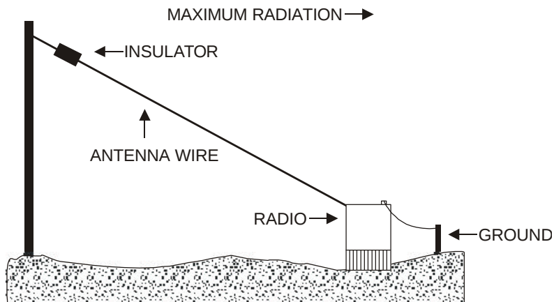
Figure 4-26. Sloping Wire.
