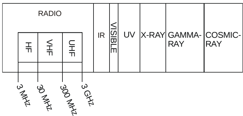
Figure 1-1. Electromagnetic Spectrum.
