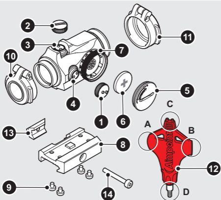
Fig. 1 Overview (configuration)
