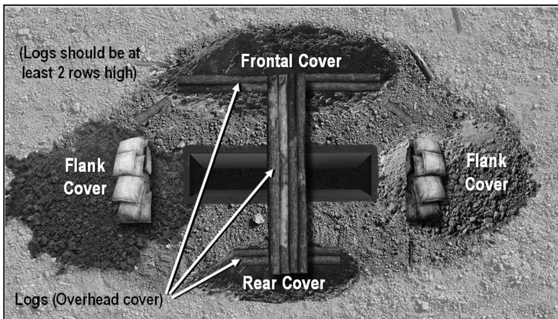
Figure 4-7. Step 4 of Fighting Position Preparation: Construction of Overhead Cover.
