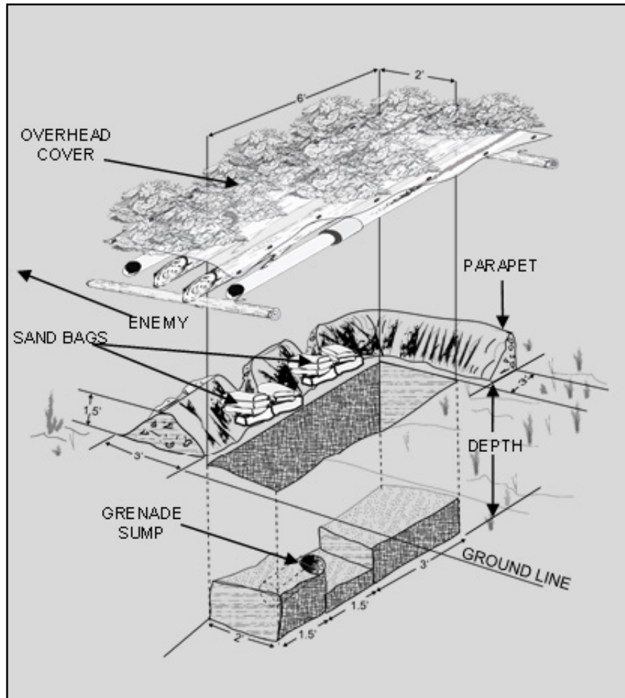
Figure 4-5. Two-Person Fighting Position.
