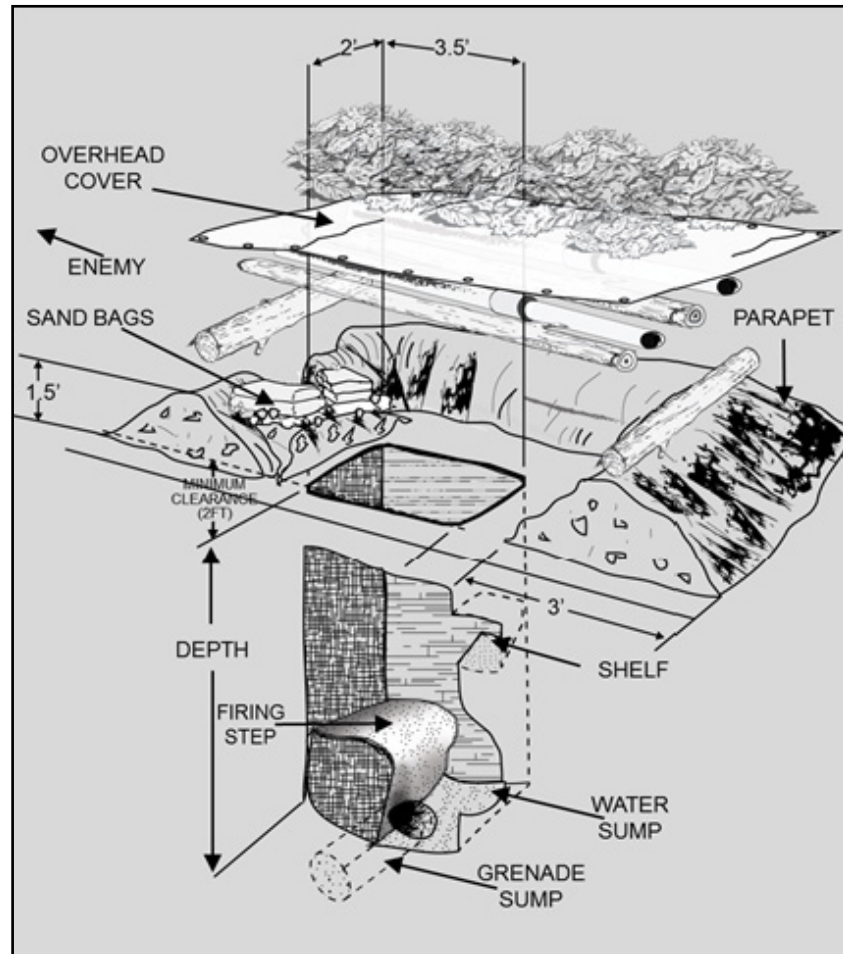
Figure 4-4. Individual Fighting Position.
