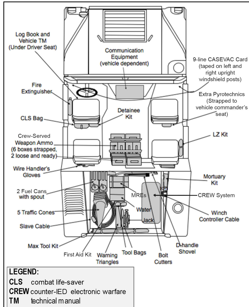
Figure 7-1. Example HMMWV Interior Packing and Load Plan.
