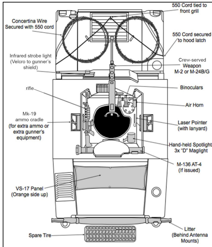
Figure 7-2. Example HMMWV Exterior Packing and Load Plan.
