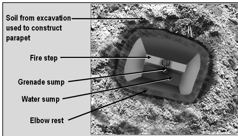
Figure 4-6. Step 3 of Fighting Position Preparation (overhead view).
